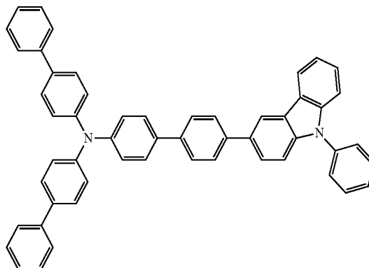
BH-1
