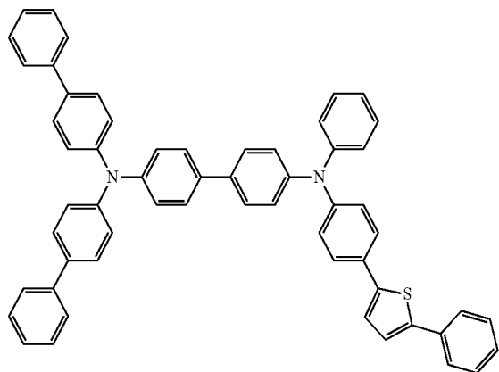
HT-1
