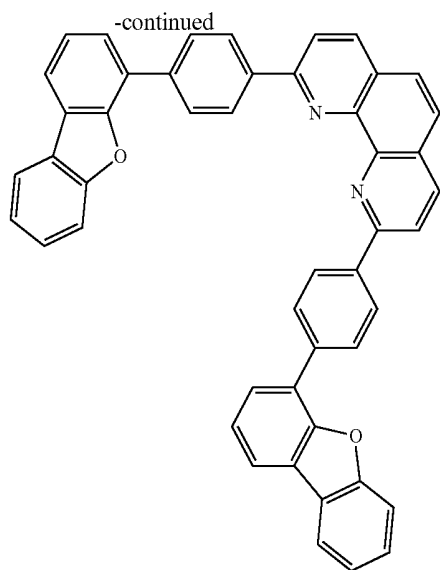
Compound 5
