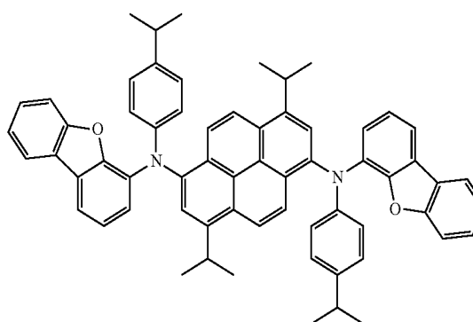
BD-1
