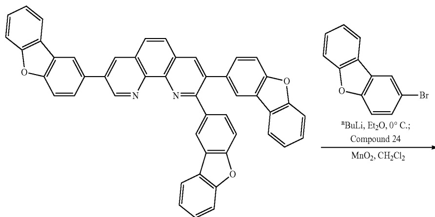
Compound 25
