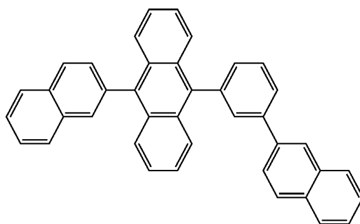
BD-1
