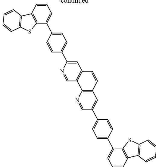
Compound 22
